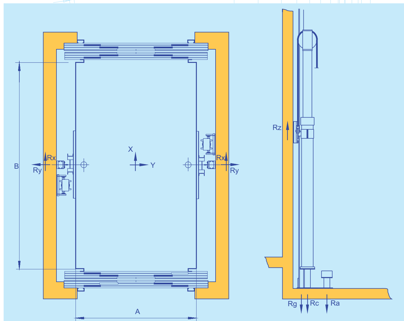
Figure 9: Schémas reactions sur gaine
